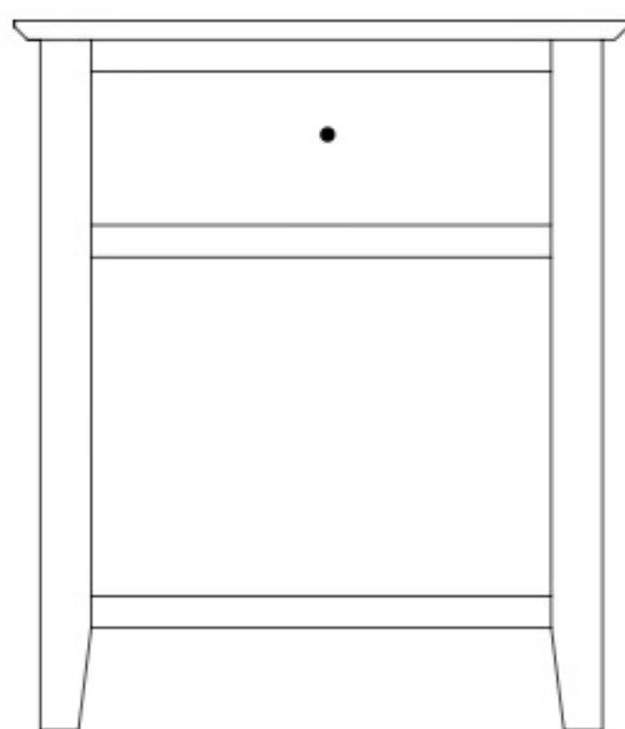
SH-2014 Night Stand 24"w 27 3/4"h 18"d w/1 drawer
