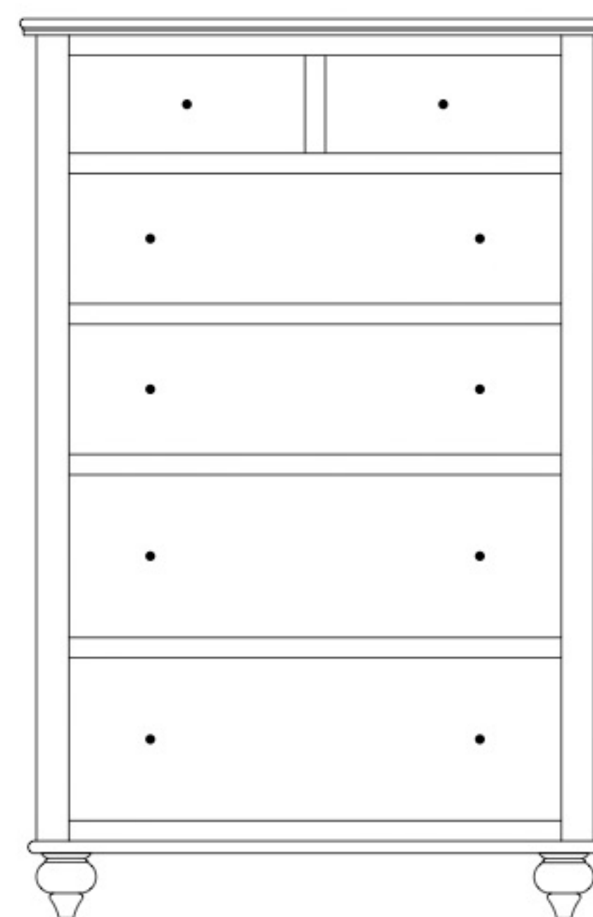
WB-1750 Chest 36 1/4"w 55 1/4"h 21"d w/6 drawers
