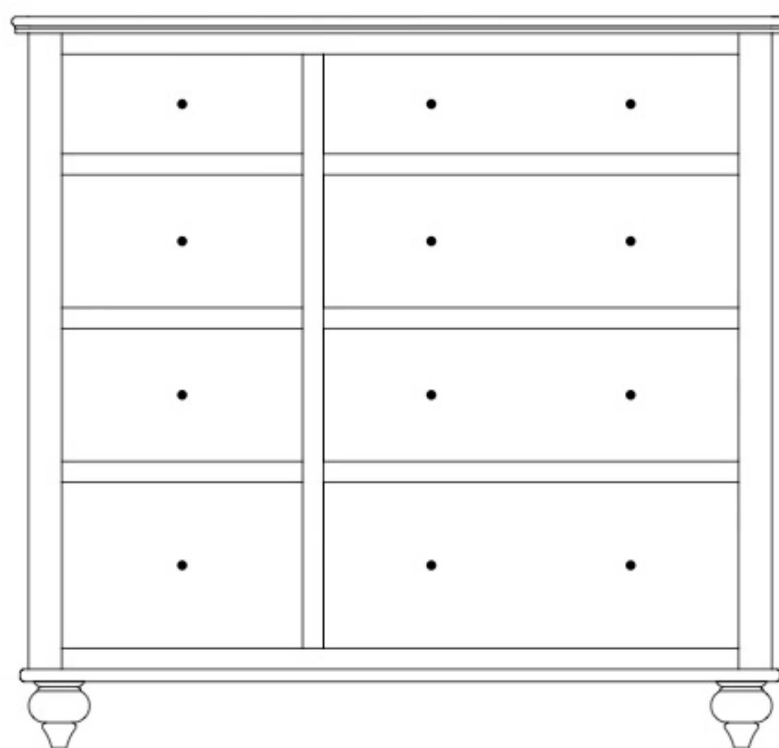
WB-1748 Chest 46 3/4"w 44"h 21"d w/8 drawers
